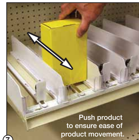
6 Position Pusher Track for optimal self-facing. Set Dividers to desired position (See step 5).
